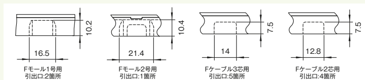
BPN-120URH PW
