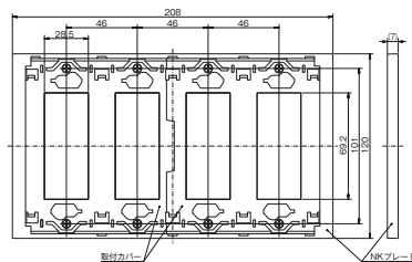
NKP-3UF-4
