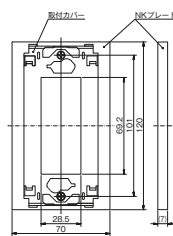
NKP-3UF-4
