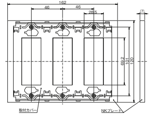
NKP-3UF-3
