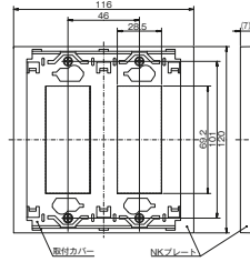
NKP-3UF-5
