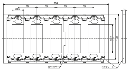
NKP-3UF-5
